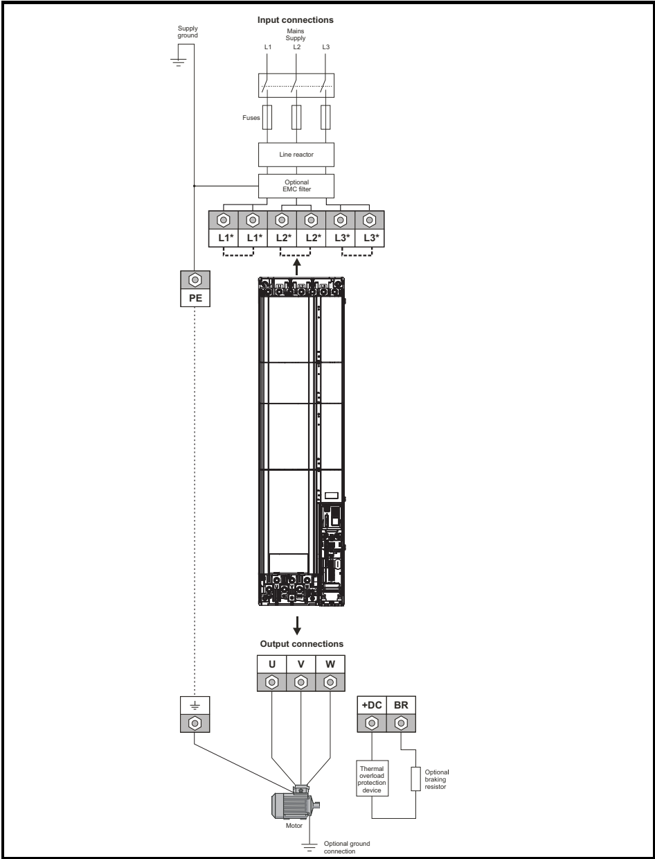
Figure 4-1 Power connections
